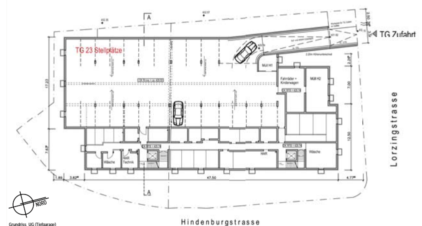
Grundriss UG (Garage)
