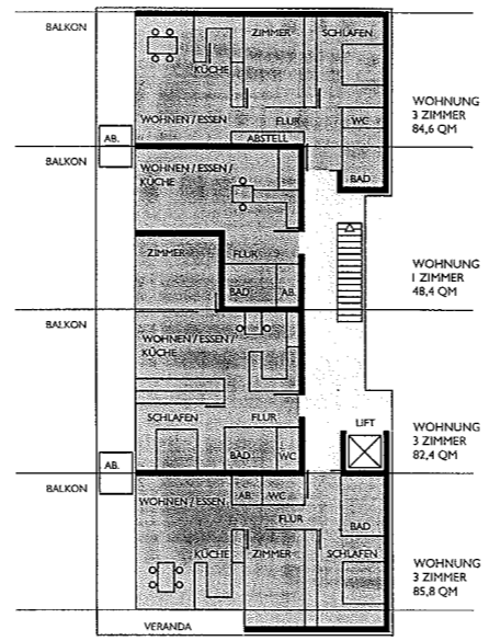
Grundriss Alternative 1
